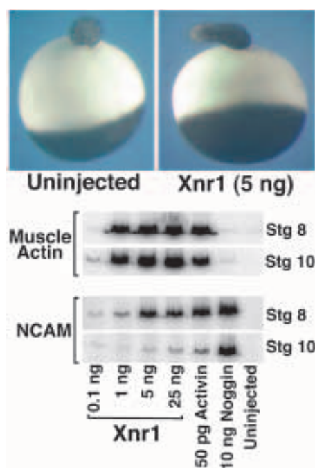
Fig. 6. Mesoderm induction is due to non-cell-autonomous signaling by Xnr1. Ectodermal explants from early blastula or early gastrula embryos were grafted onto uninjected oocytes or onto oocytes injected with the indicated amount of Xnr1, activin, or noggin RNA. Upper panel: oocyte-explant conjugates were photographed when sibling embryos reached the early tailbud stage. Lower panels: explants were detached from the oocytes when sibling embryos reached the early tailbud stage, and then assayed by RT-PCR for expression of the mesodermal marker muscle actin or the neural marker NCAM. Each sample consisted of a pooled set of six explants, and each PCR reaction contained the cDNA equivalent of one-tenth of an explant.
